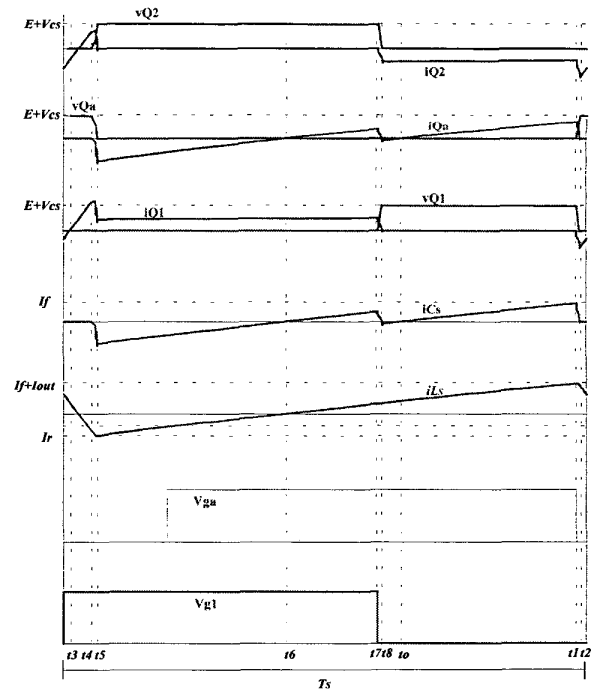
Fig. 2. Main Waveforms.
