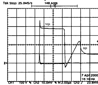
Fig. 6. Voltage and current in Q1, D1 e C1 100V/div, 50A/div, 2us/div
