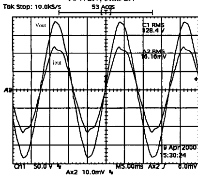
Fig. 11. Output voltage and current 50V/div, 50A/div, 5ms/div
