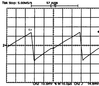
Fig. 9. Current in Ls 50A/div, 10us/div
