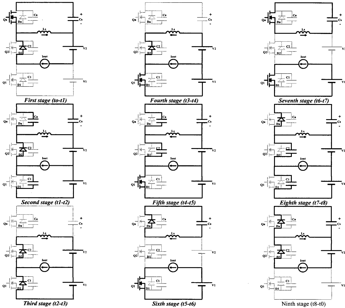
Fig. 3. Operation Stage
