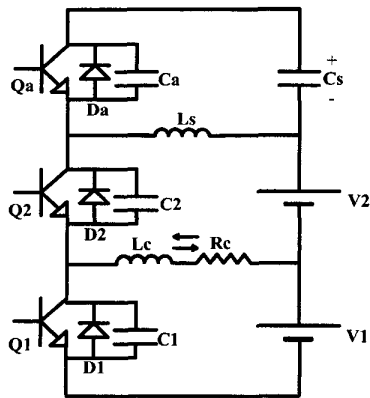
Fig. 1. Proposed Circuit.
