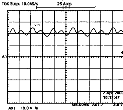
Fig. 10. Voltage in Cs 10V/div, 5ms/div
