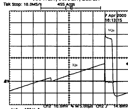
Fig. 8. Voltage and current in Qa, Da e Ca 100V/div, 50A/div, 10us/div
