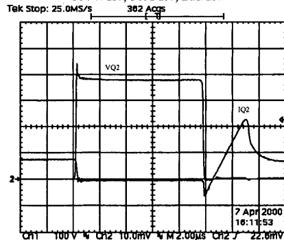
Fig. 7. Voltage and current in Q2, D2 e C2 100V/div, 50A/div, 2us/div
